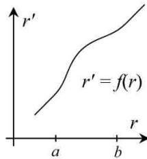
Fig. 1: The coordinate change r' = f(r) : r' = r except in the hole a < r < b .
