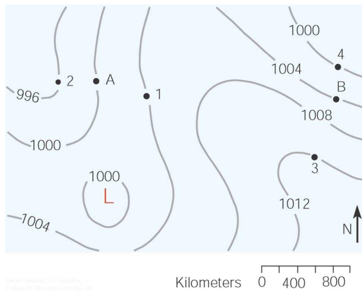
Figure 1: Sea-level pressure chart.
